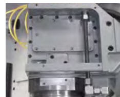
Example milling head of a DMU 125 P duoBLOCK
